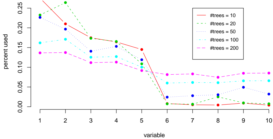
Figure 5: Average use per splitting rule for variables x_1, \dots, x_{10} when m = 10, 20, 50, 100, 200 .
