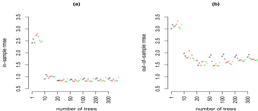
Figure 6: BART’s robust RMSE performance as (\nu, q, k, m) is varied: (a) in-sample RMSE comparisons and (b) out-of-sample RMSE comparisons. (Horizontal jittering of points has been used to improve readability).
