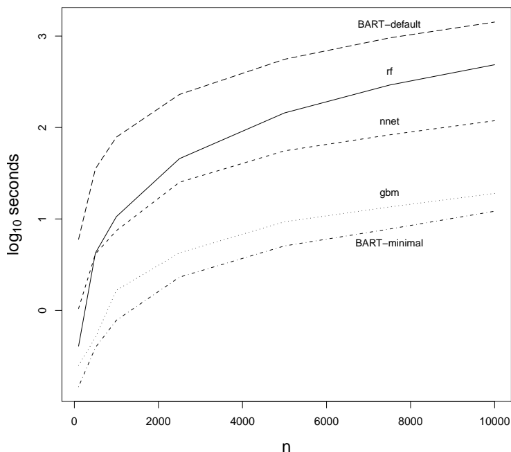
Figure 12: Execution time comparisons of various methods, with \log_{10} seconds plotted versus sample size n = 100, 500, 1000, 2500, 5000, 7500, 10000 .
